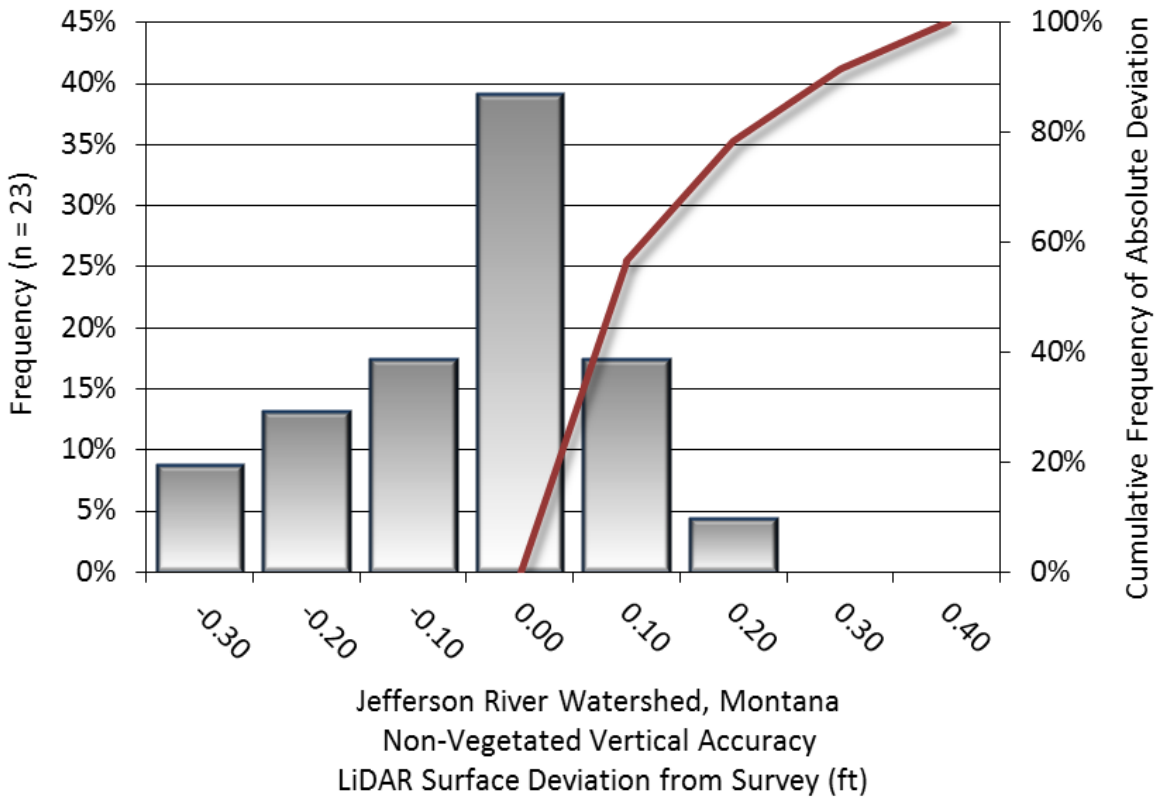
Figure 10: Frequency histogram for LiDAR surface deviation from ground check point values (NVA)
