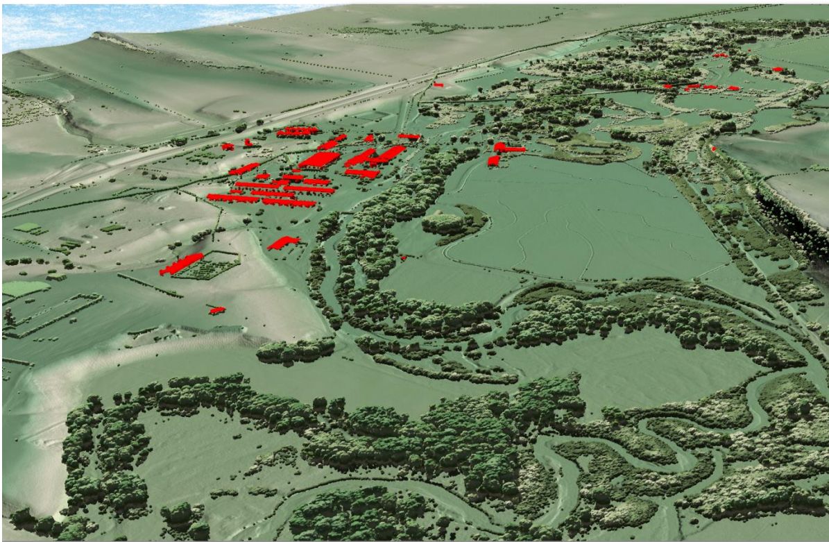
Figure 5: This image shows a view of the building classification in the Musselshell and Wheatland Counties site, created from the bare earth model colored by elevation, and overlaid with the above-ground point cloud colored by point classification.
