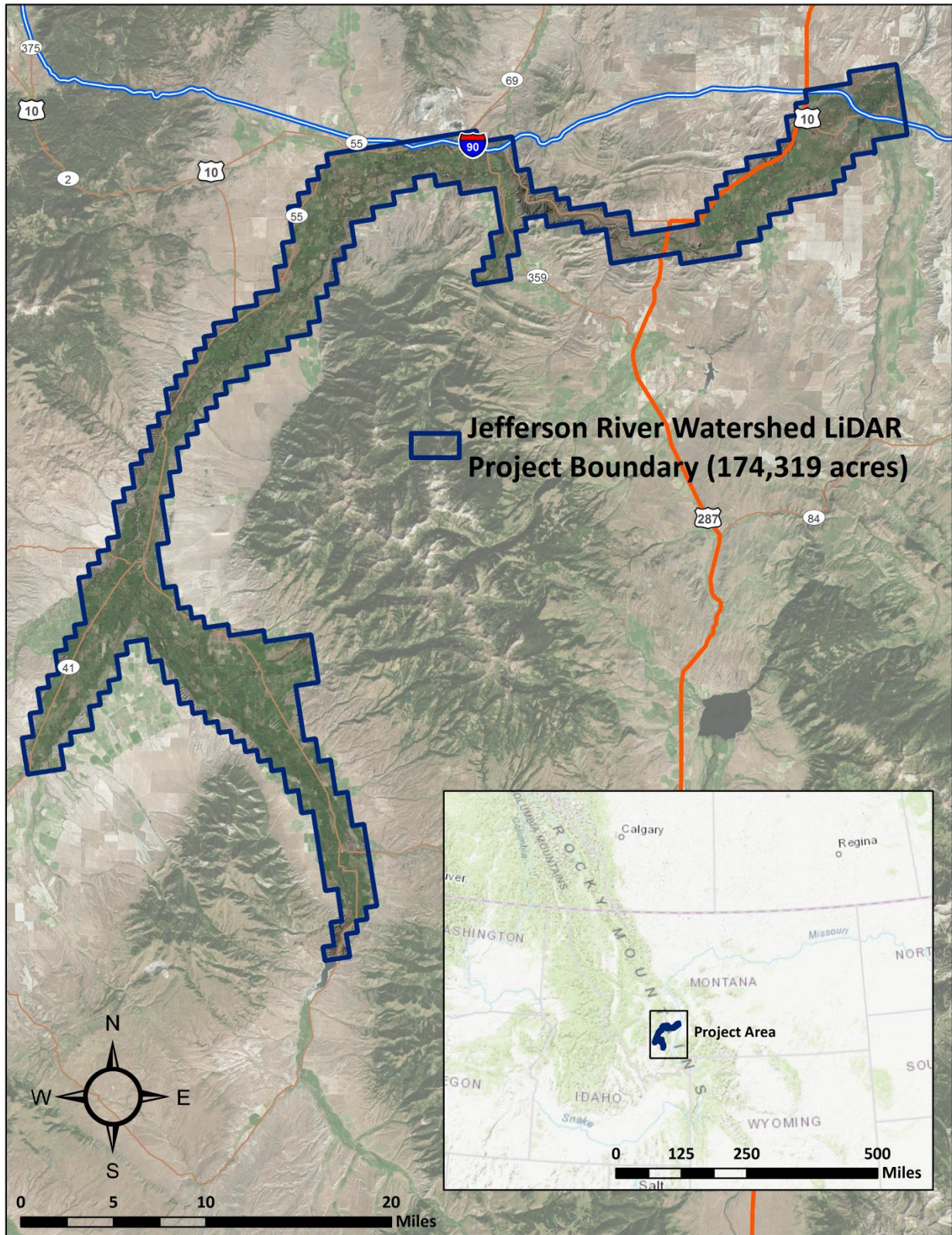
Figure 1: Location map of the Jefferson River Watershed site in Montana
