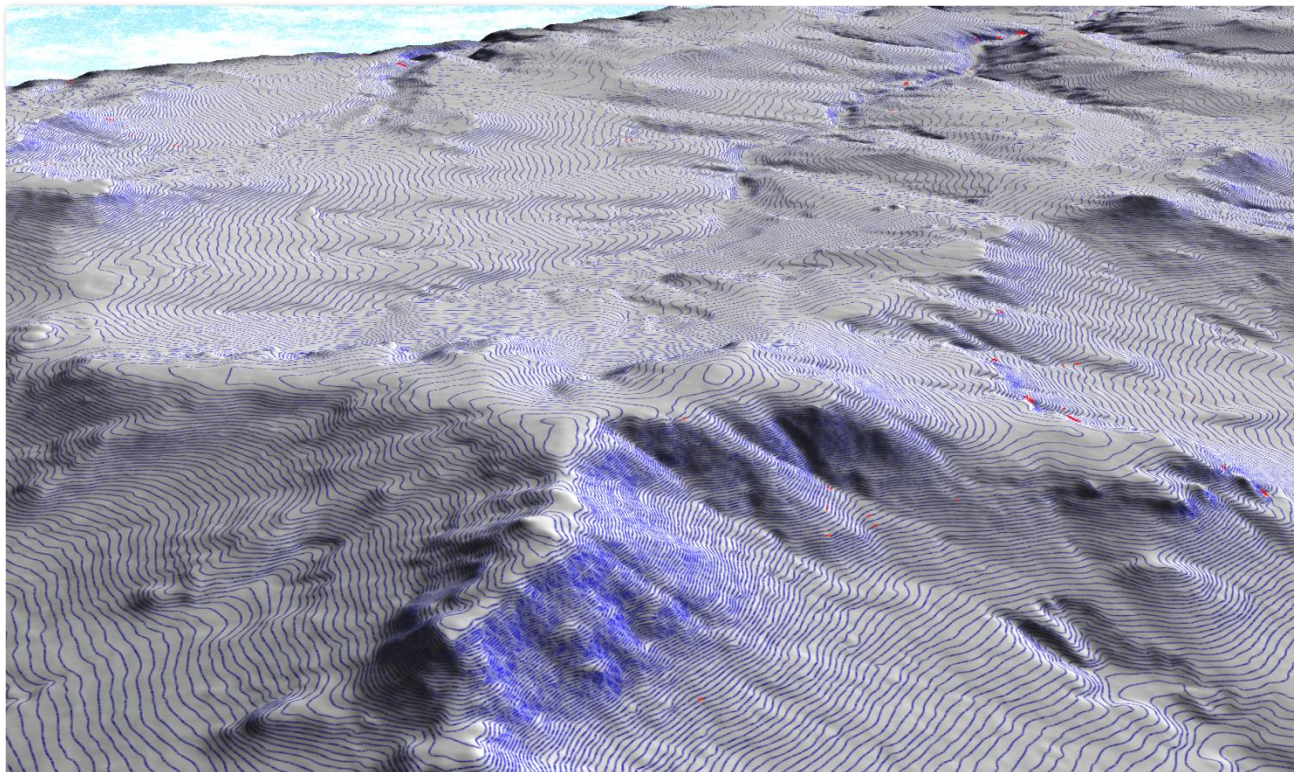
Figure 4: Contours draped over the bare earth elevation model in one of the MTDNRC project sites. Blue contours represent high confidence while the red contour segments represent low confidence.
