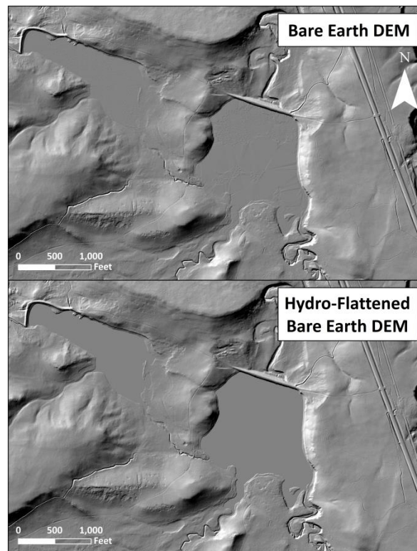
Figure 3: Example of hydroflattening in MTDNRC project sites
