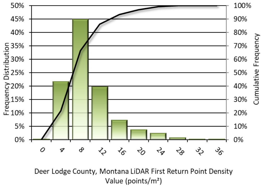
Figure 6: Frequency distribution of Deer Lodge County QL2 first return point density values per 100 x 100 m cell
