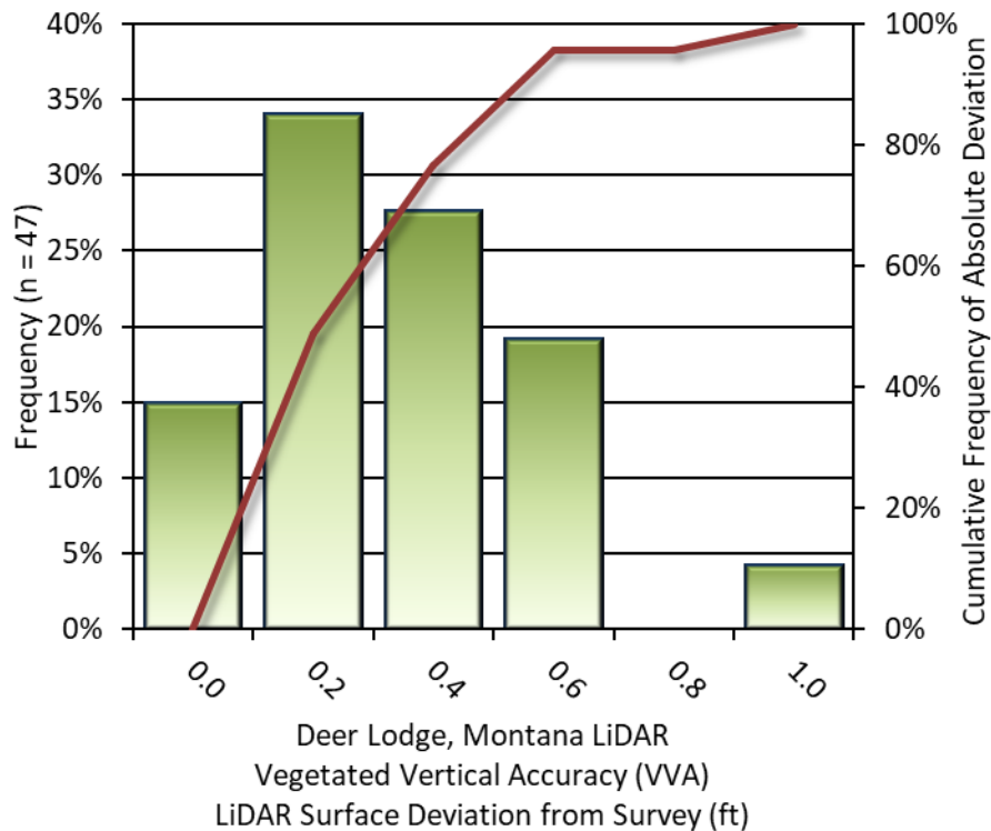
Figure 13: Frequency histogram for LiDAR surface deviation from vegetated check point values (VVA)
