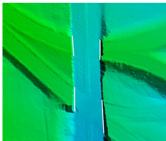
Figure 5: This image shows proper classing and handling of bridges in a bare earth surface model. The white line features are bridge breaklines that enforce ground elevations along the elevated sides of the removed bridge deck. Bridge breaklines prevent 'saddles' and enforce a logical terrain surface beneath the bridge.
