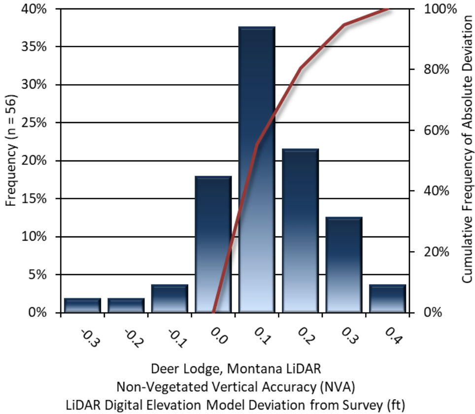
Figure 11: Frequency histogram for LiDAR bare earth DEM surface deviation from ground check point values (NVA)
