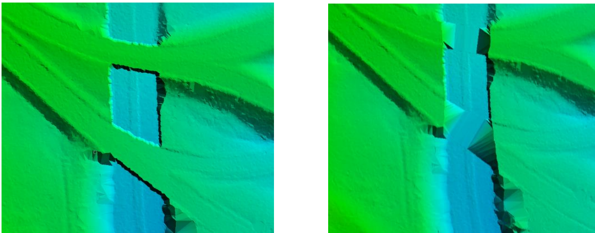
Figure 4: The image to the left depicts a bare earth surface model with two bridges improperly classified as ground. The image to the right shows two bridges properly classed to Class 17, however bridge classing artifacts called 'saddles' are present.
