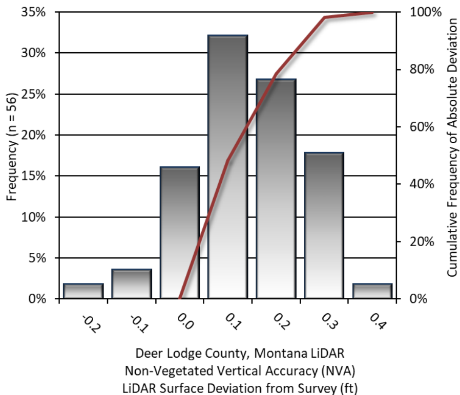
Figure 10: Frequency histogram for LiDAR unclassified LAS deviation from ground check point values (NVA)
